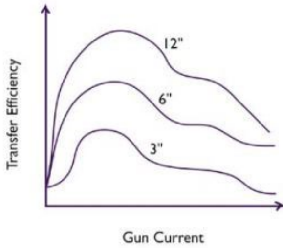
Transfer Efficiency vs. Gun to Part Distance
